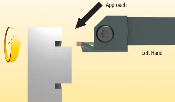
Clockwise Rotation Square Shank
